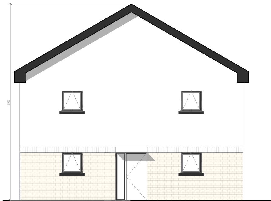
SIDE ELEVATION 2 BEDROOM ALTERNATIVE
